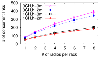
(a) Impact of # of Radios per Rack
